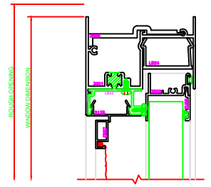
100 HEAD SERIES: 3500
